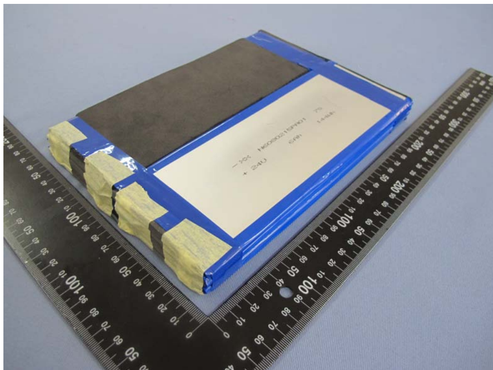
Fig.1 Overall view I of cell pack
