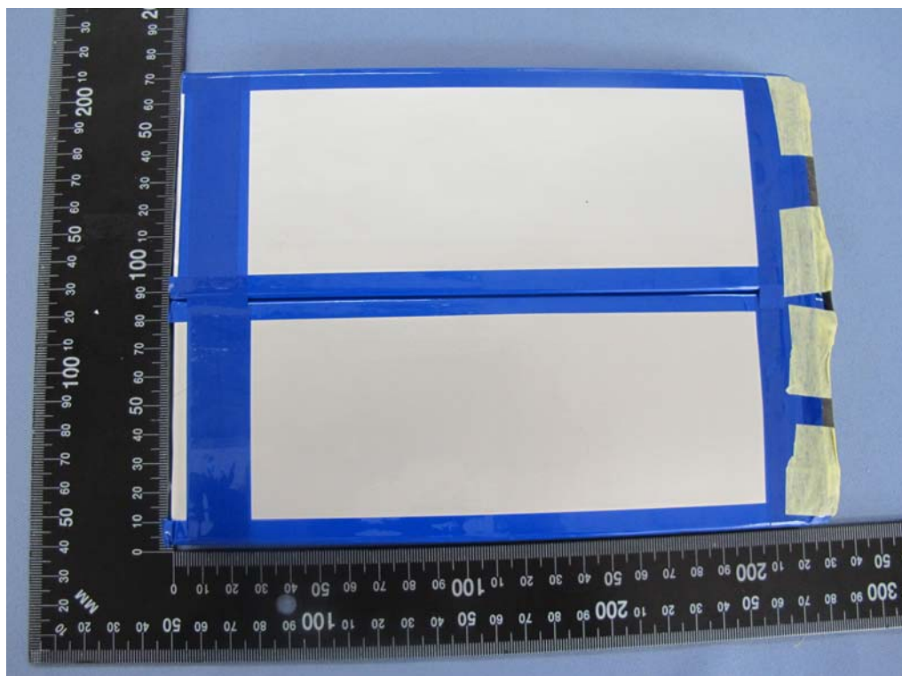
Fig.2 Overall view II of cell pack
